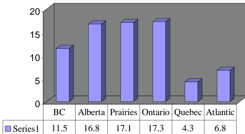
Fig. 4 - Percentage of SCMs to the quantity of cement used in each region (2001).
